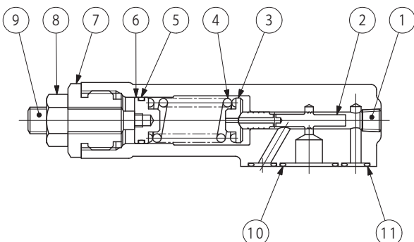
Pressure compensator mechanism parts
